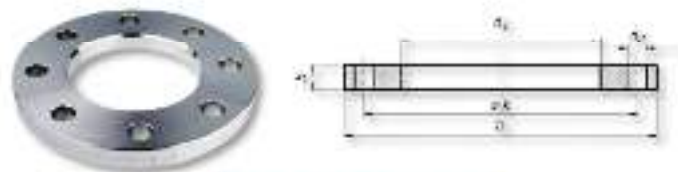
Flat Face Flange
