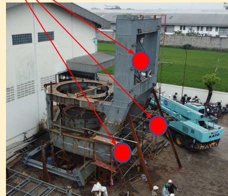
Vertical Holding Platform
