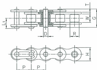
Standard Type (Roller chain)
