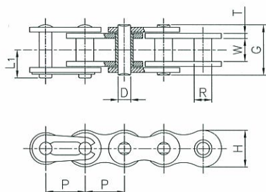
Standard Type (Bushing chain)
