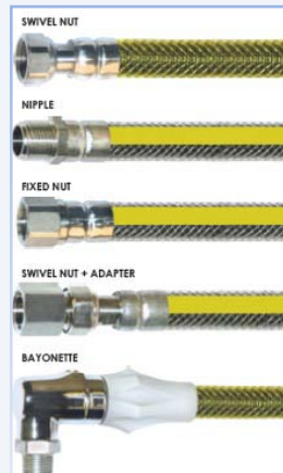
GAS HOSES
