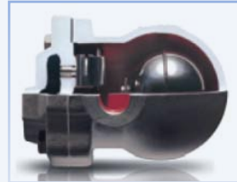
FLOAT TYPE STEAM TRAPS WITH AIR VENT SK-51/SK-51C
