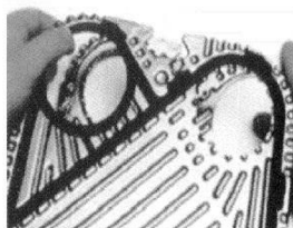
Plates & Gaskets
