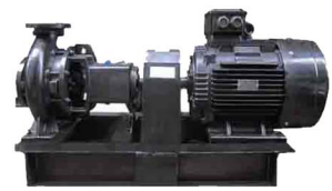
Centrifugal End Suction Pump Couple With Motor
