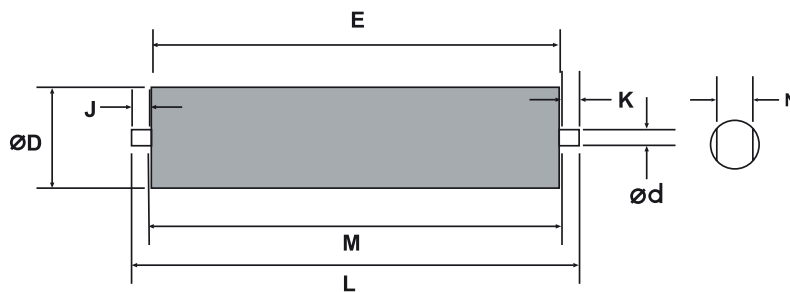
ROLLER DIMENSION
