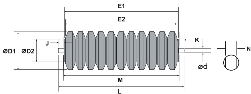
ROLLER DIMENSION
