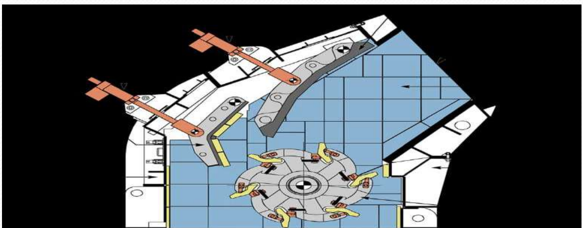
Liner/Dinding Crusher
