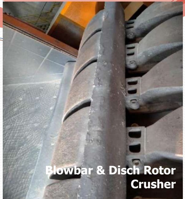
Rotor Impact Crusher
