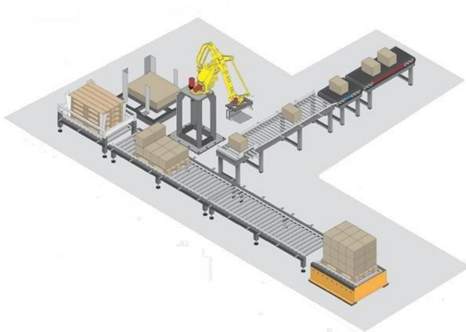
Robot Palletizer Lay Out Example
