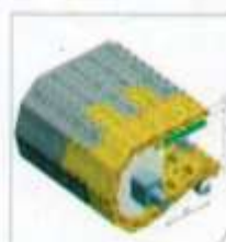
Type 型号: HS-1800B Pitch 节距: 63.5MM Thickness 厚度: 25MM Open area 开孔率: 10%
