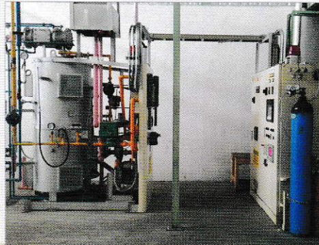
Induction Machine
