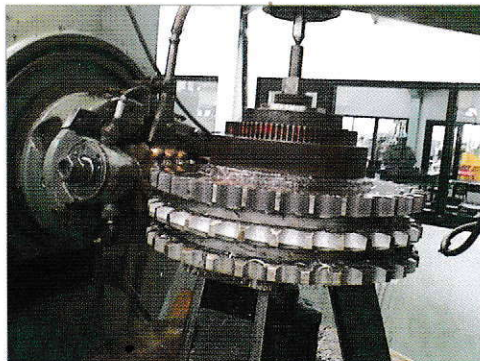
CNC Machine
