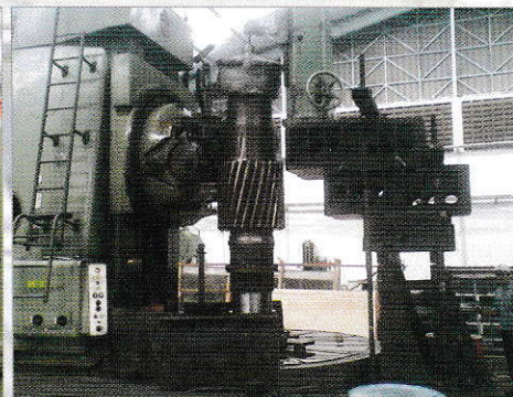
Hobbing Machine
