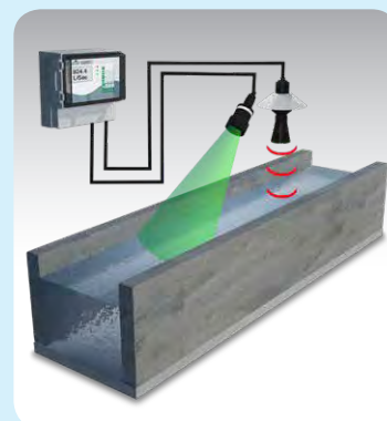
Microflow and Flowcert Channel
