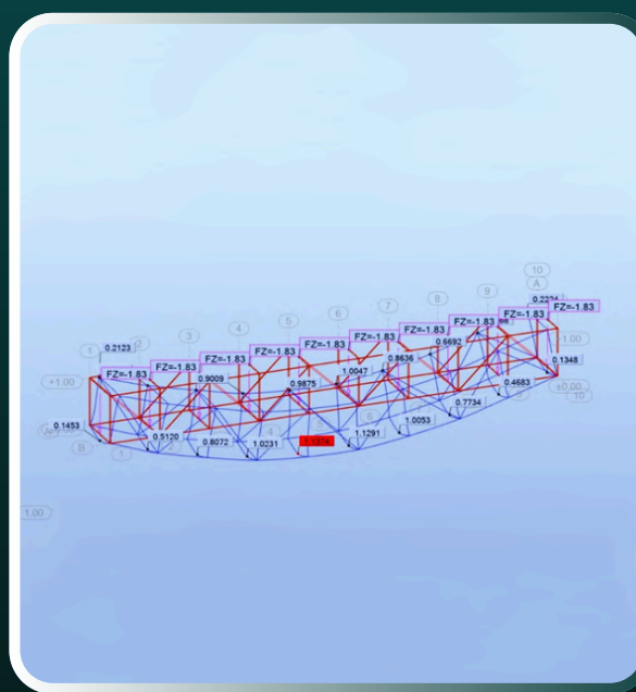
STEEL STRUCTURE ANALYSIS CIVIL WORK
