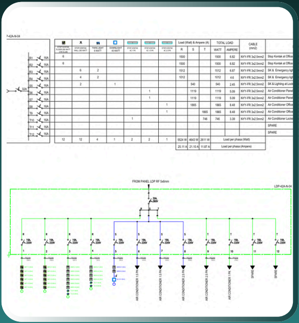
SINGLE LINE DIAGRAM ELECTRICAL WORK
